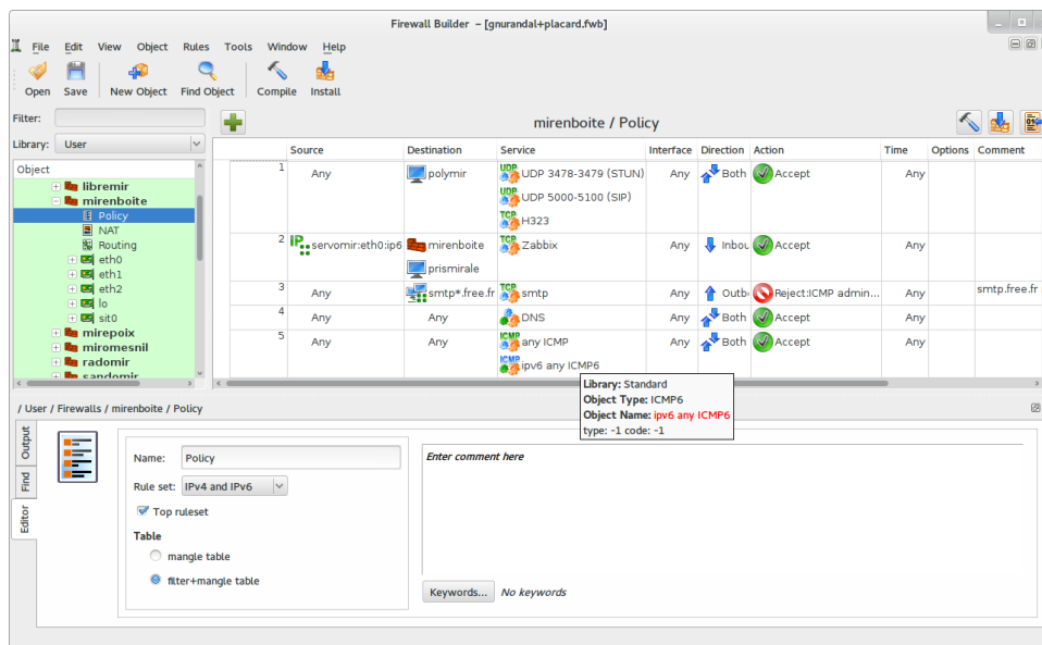
FIGURE 14.2 Fwbuilder en action
